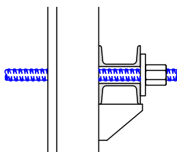
Spundwandverankerung sheet pile anchorage
